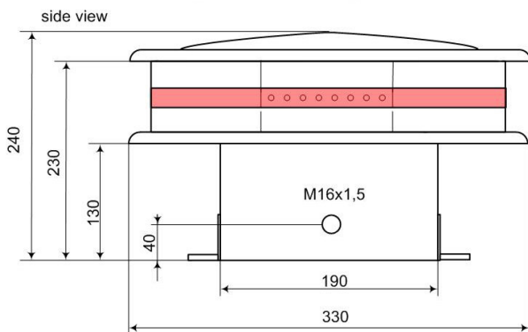
Medium intensity obstruction light AOL 303
